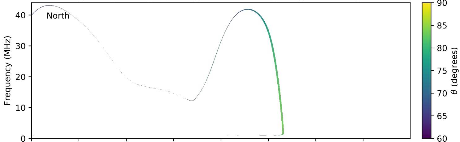
expres_earth_jupiter_io_jrm09_lossc-wid1deg_3kev_20121231_v01.cdf
