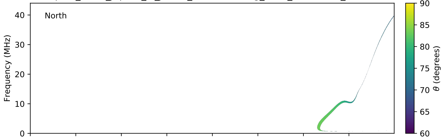
expres_earth_jupiter_io_jrm09_lossc-wid1deg_3kev_20121230_v01.cdf
