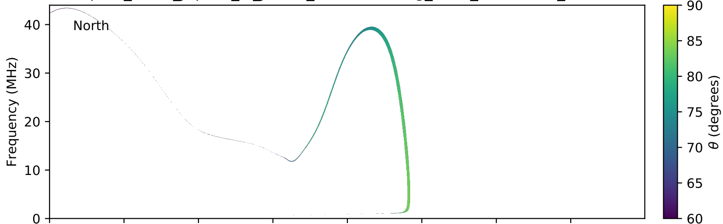
expres_earth_jupiter_io_jrm09_lossc-wid1deg_3kev_20121224_v01.cdf
