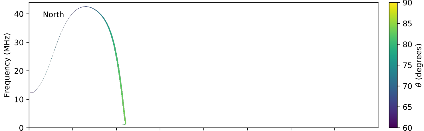
expres_earth_jupiter_io_jrm09_lossc-wid1deg_3kev_20121219_v01.cdf
