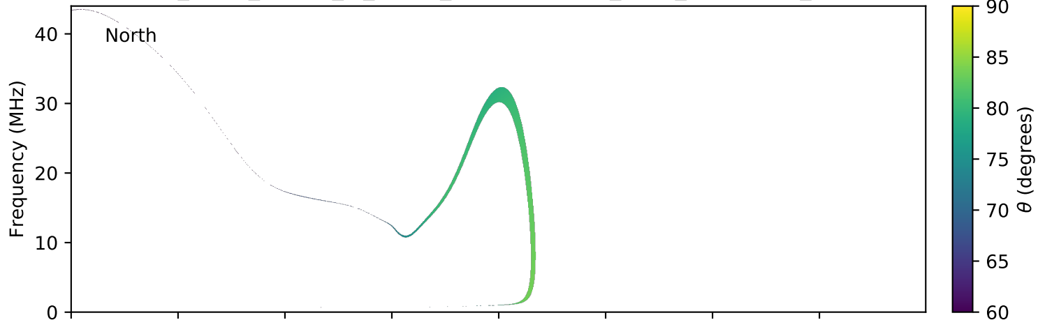
expres_earth_jupiter_io_jrm09_lossc-wid1deg_3kev_20121217_v01.cdf
