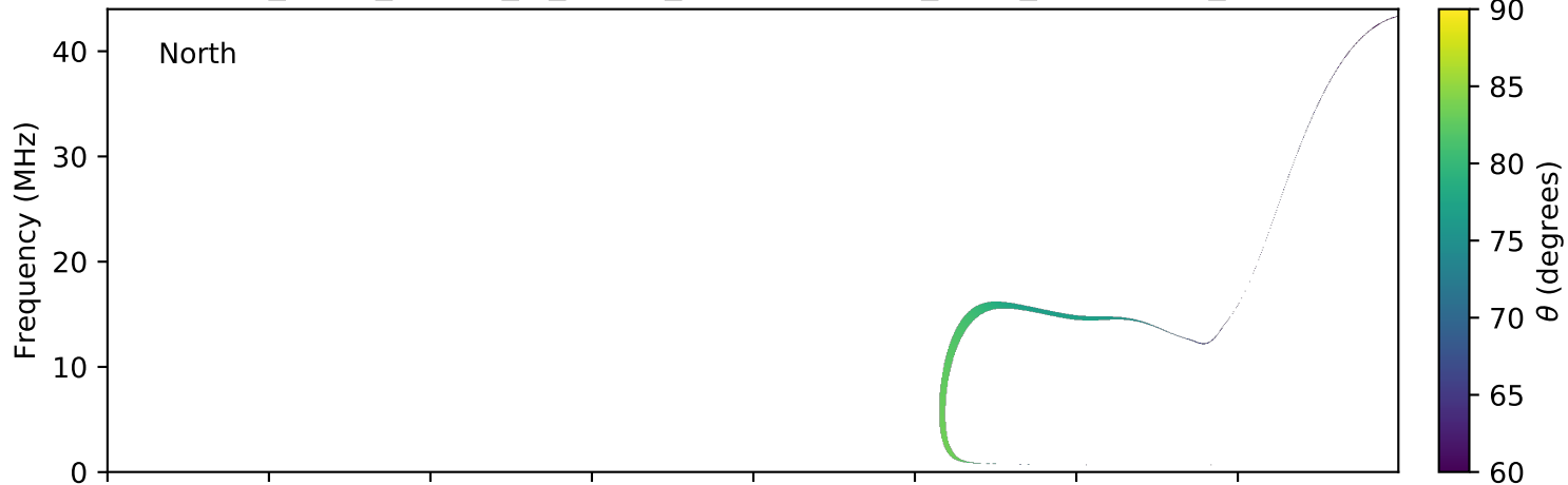
expres_earth_jupiter_io_jrm09_lossc-wid1deg_3kev_20121216_v01.cdf
