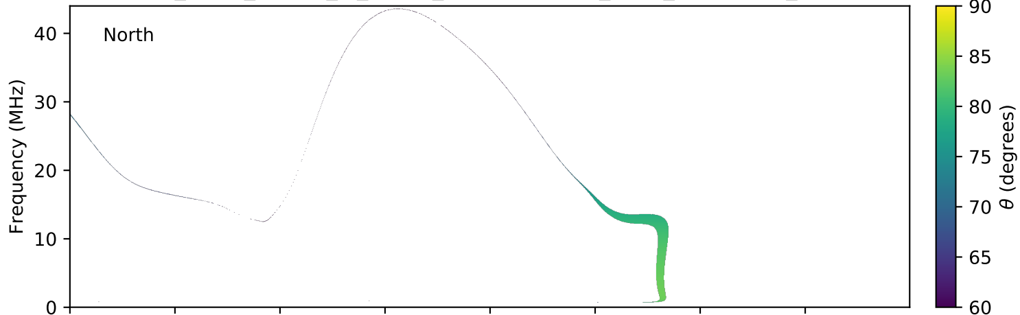
expres_earth_jupiter_io_jrm09_lossc-wid1deg_3kev_20121215_v01.cdf
