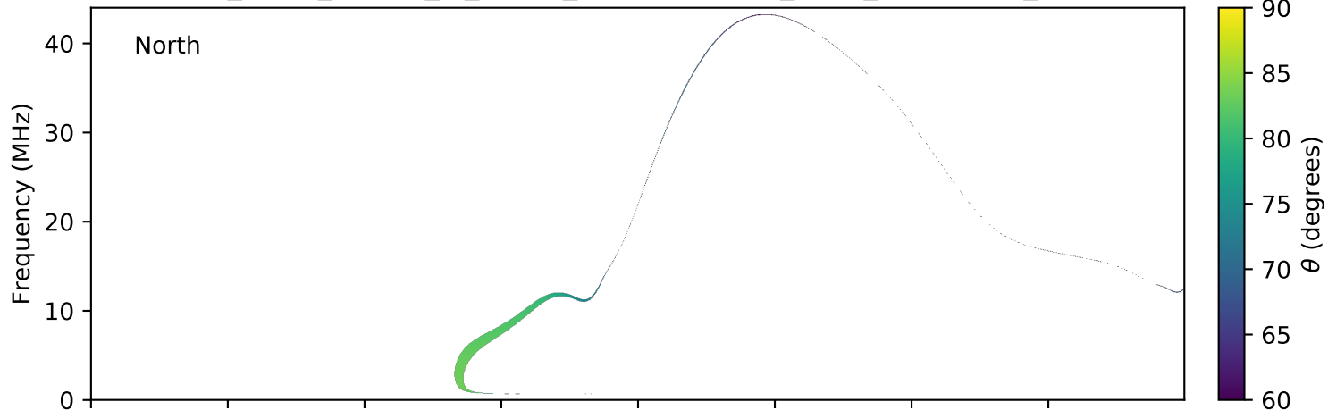
expres_earth_jupiter_io_jrm09_lossc-wid1deg_3kev_20121211_v01.cdf
