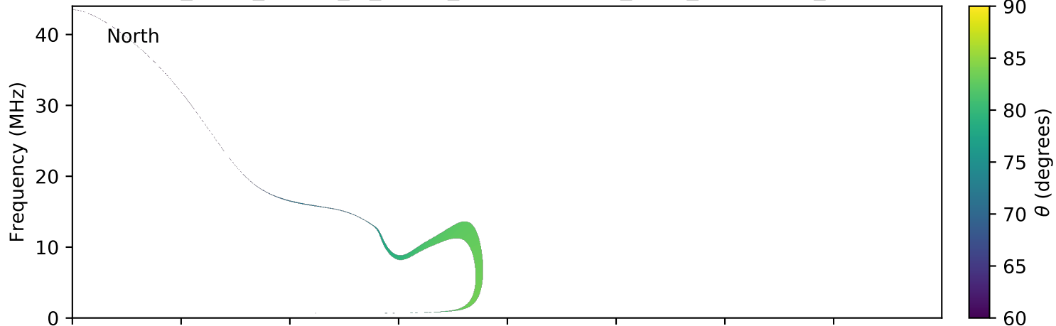
expres_earth_jupiter_io_jrm09_lossc-wid1deg_3kev_20121210_v01.cdf
