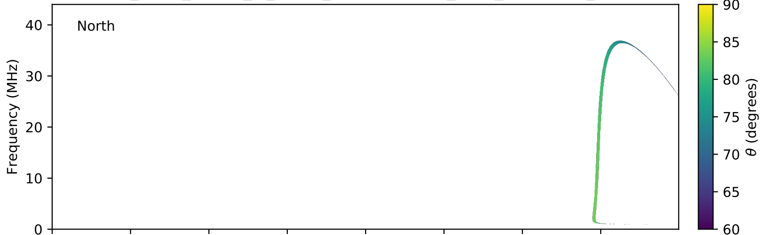
expres_earth_jupiter_io_jrm09_lossc-wid1deg_3kev_20121207_v01.cdf
