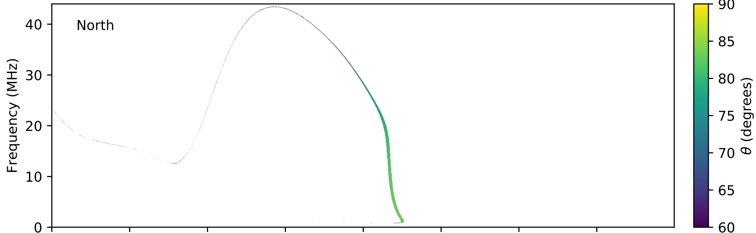
expres_earth_jupiter_io_jrm09_lossc-wid1deg_3kev_20121201_v01.cdf
