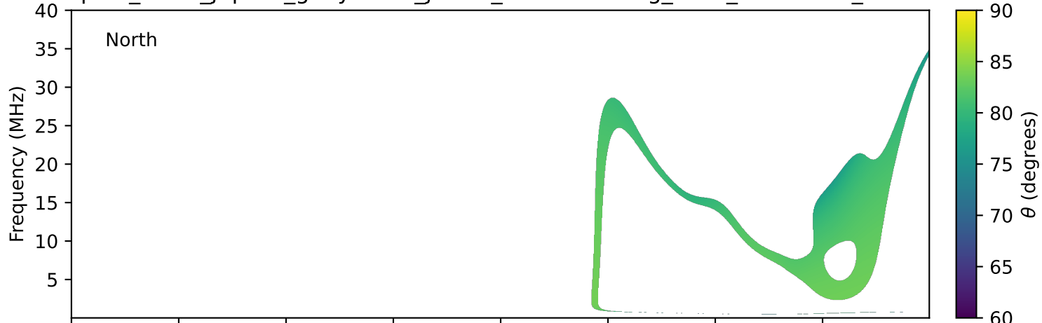
expres_earth_jupiter_ganymede_jrm33_lossc-wid1deg_3kev_20121211_v11.cdf
