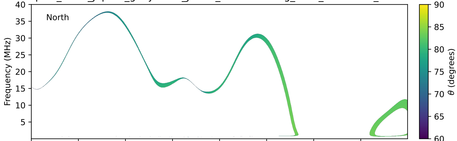
expres_earth_jupiter_ganymede_jrm33_lossc-wid1deg_3kev_20121207_v11.cdf
