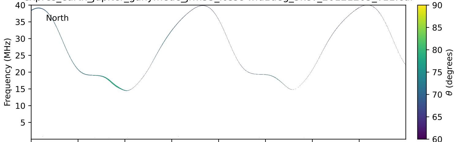
expres_earth_jupiter_ganymede_jrm33_lossc-wid1deg_3kev_20121205_v11.cdf
