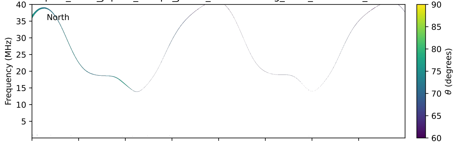
expres_earth_jupiter_europa_jrm33_lossc-wid1deg_3kev_20121224_v11.cdf
