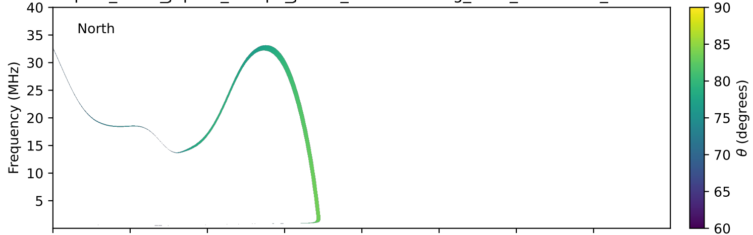
expres_earth_jupiter_europa_jrm33_lossc-wid1deg_3kev_20121218_v11.cdf
