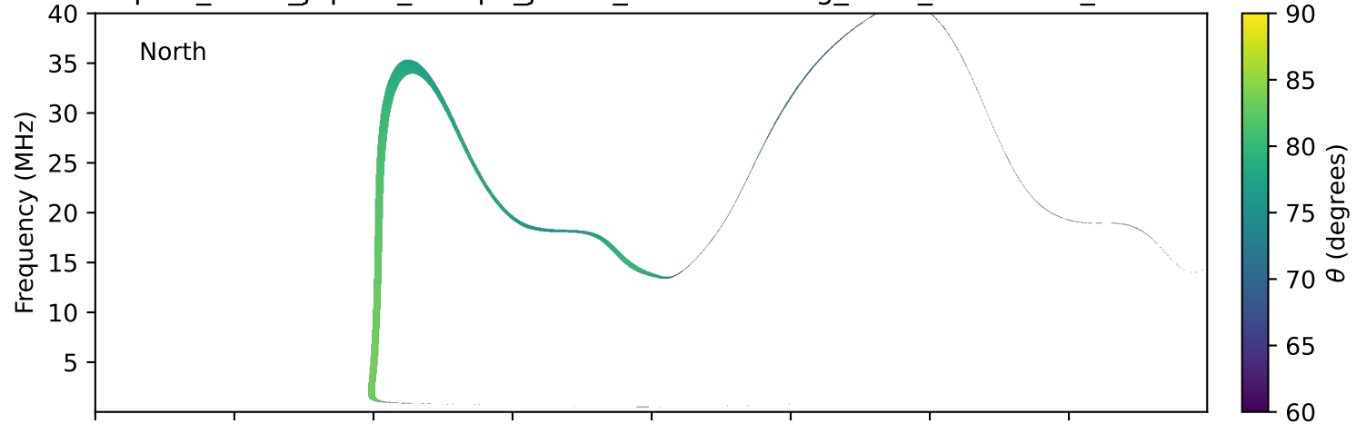
expres_earth_jupiter_europa_jrm33_lossc-wid1deg_3kev_20121213_v11.cdf
