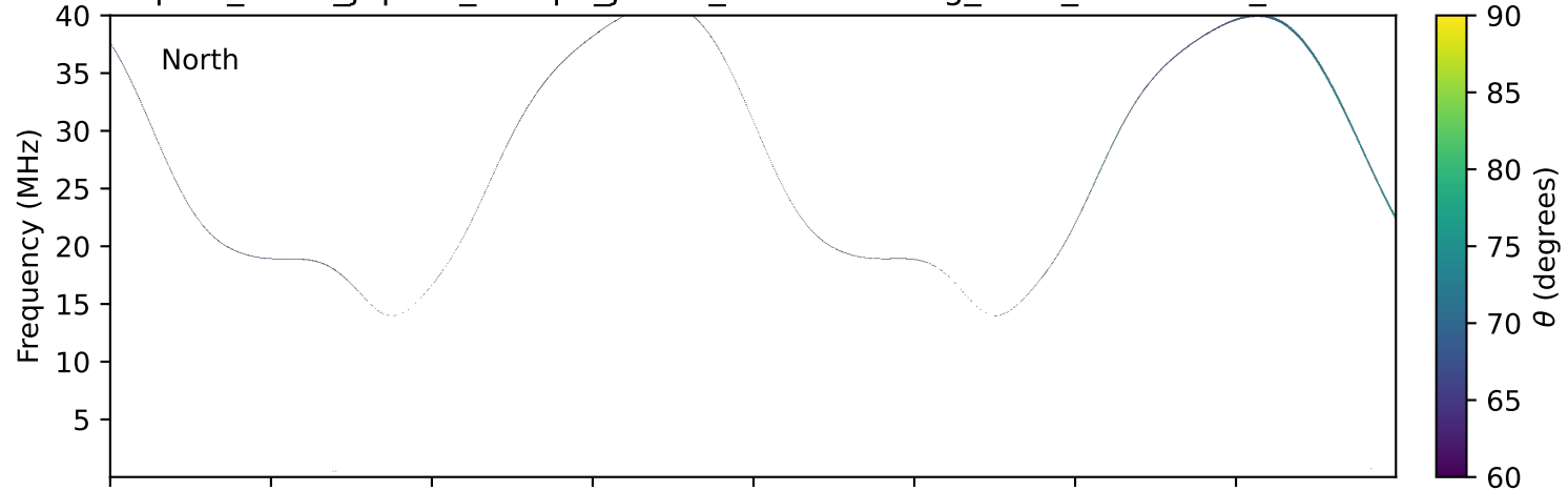
expres_earth_jupiter_europa_jrm33_lossc-wid1deg_3kev_20121203_v11.cdf
