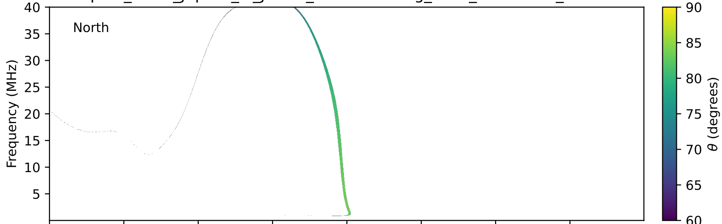
expres_earth_jupiter_io_jrm33_lossc-wid1deg_3kev_20121124_v11.cdf
