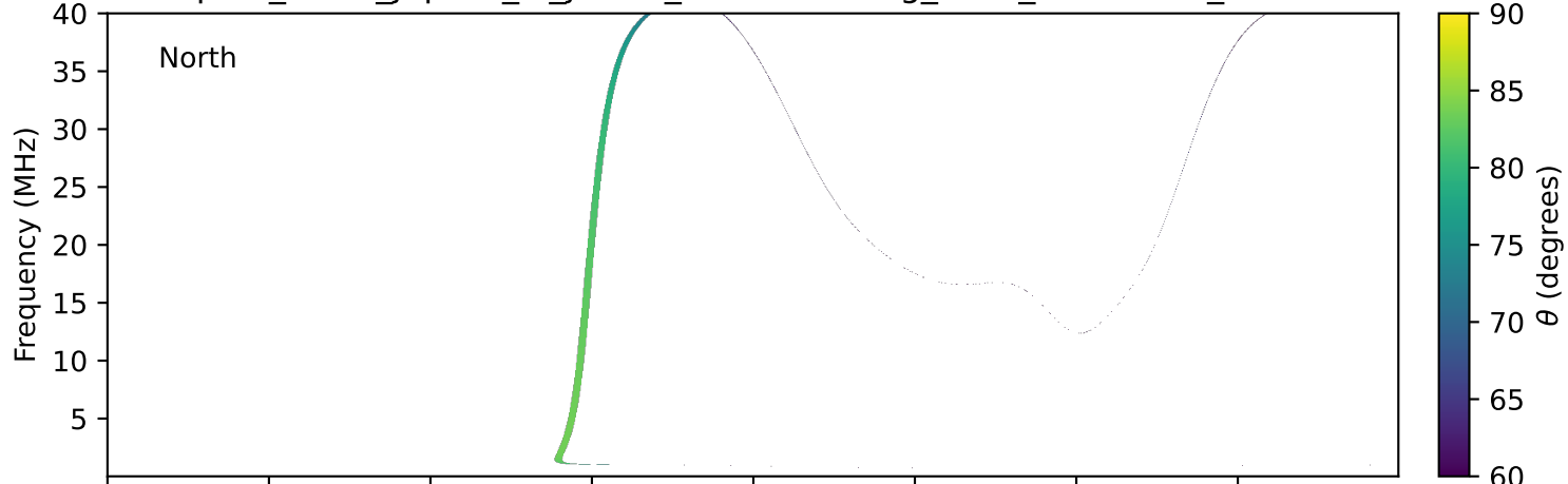
expres_earth_jupiter_io_jrm33_lossc-wid1deg_3kev_20121111_v11.cdf
