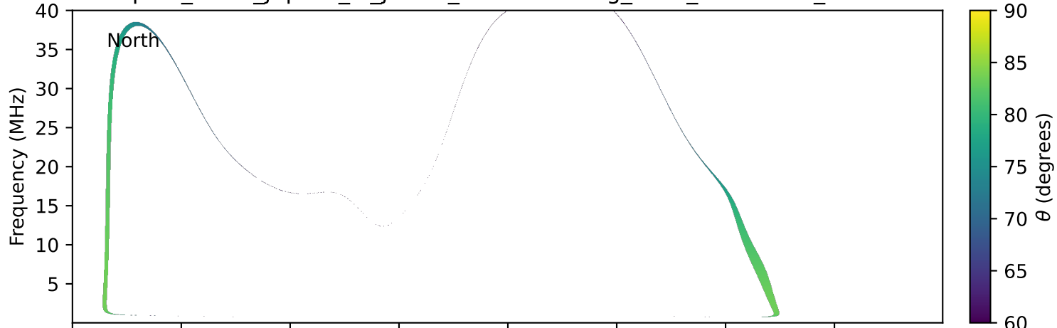
expres_earth_jupiter_io_jrm33_lossc-wid1deg_3kev_20121106_v11.cdf
