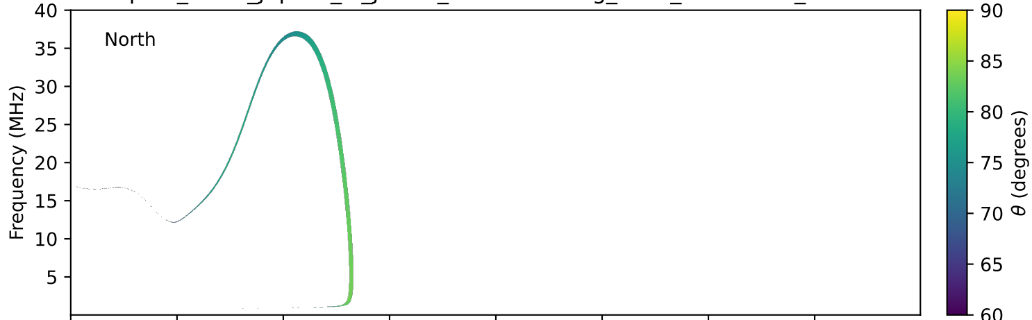
expres_earth_jupiter_io_jrm33_lossc-wid1deg_3kev_20121103_v11.cdf
