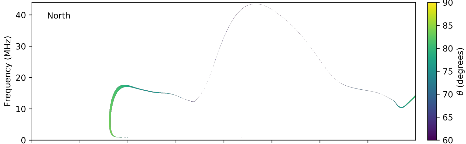
expres_earth_jupiter_io_jrm09_lossc-wid1deg_3kev_20121127_v01.cdf
