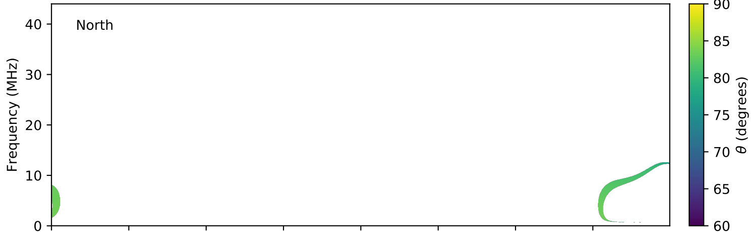
expres_earth_jupiter_io_jrm09_lossc-wid1deg_3kev_20121121_v01.cdf
