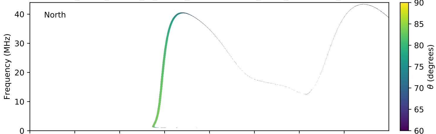
expres_earth_jupiter_io_jrm09_lossc-wid1deg_3kev_20121111_v01.cdf
