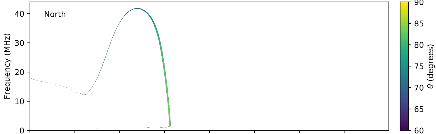
expres_earth_jupiter_io_jrm09_lossc-wid1deg_3kev_20121110_v01.cdf
