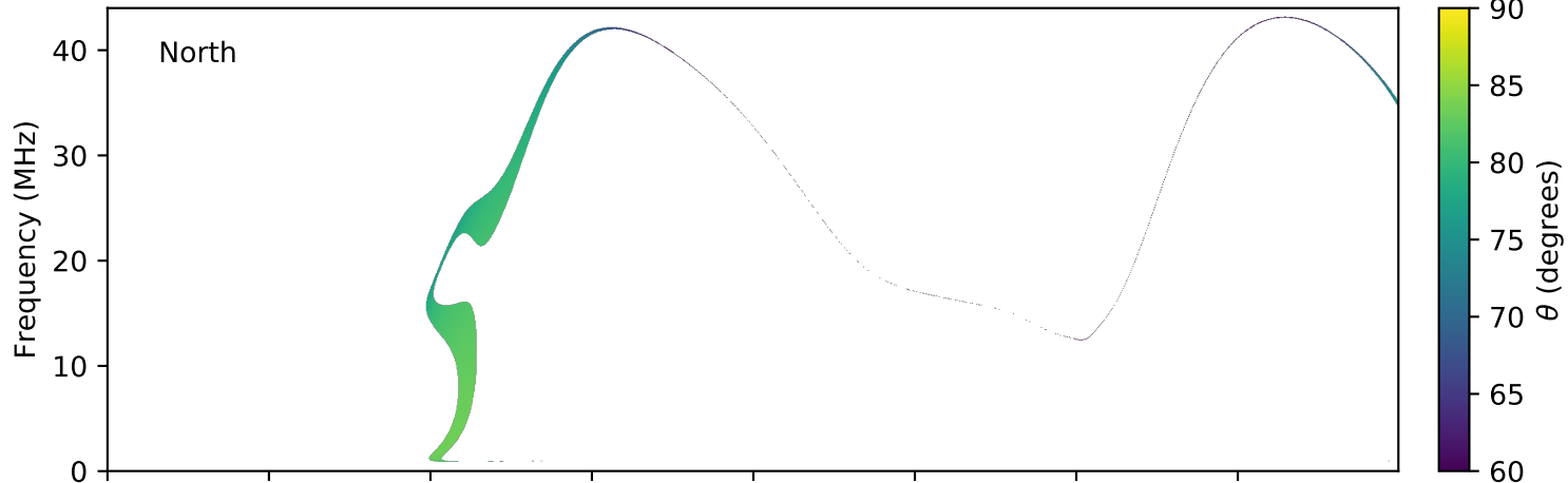
expres_earth_jupiter_io_jrm09_lossc-wid1deg_3kev_20121104_v01.cdf
