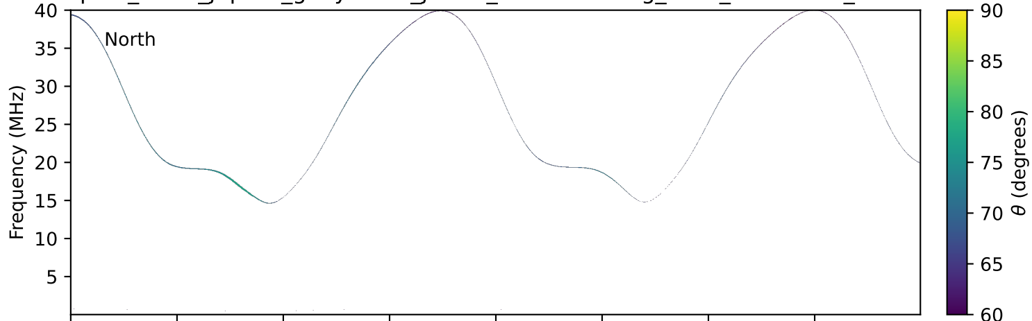
expres_earth_jupiter_ganymede_jrm33_lossc-wid1deg_3kev_20121128_v11.cdf
