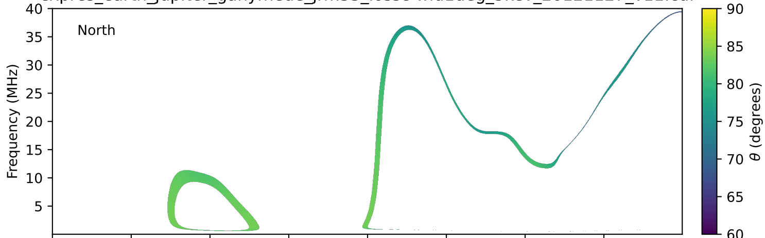
expres_earth_jupiter_ganymede_jrm33_lossc-wid1deg_3kev_20121127_v11.cdf
