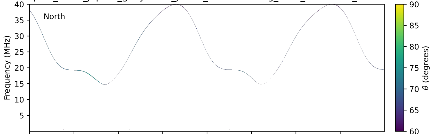
expres_earth_jupiter_ganymede_jrm33_lossc-wid1deg_3kev_20121121_v11.cdf
