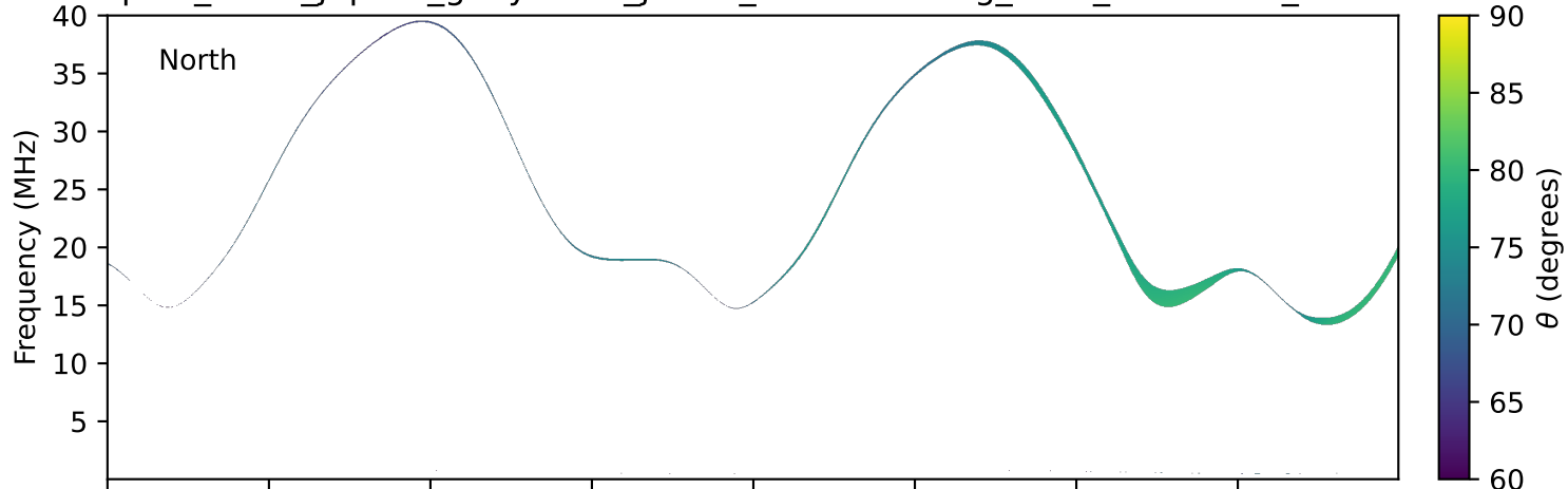
expres_earth_jupiter_ganymede_jrm33_lossc-wid1deg_3kev_20121108_v11.cdf
