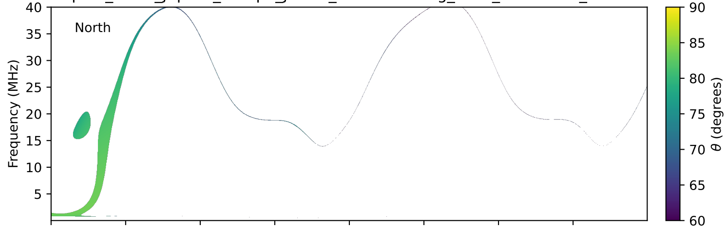
expres_earth_jupiter_europa_jrm33_lossc-wid1deg_3kev_20121122_v11.cdf
