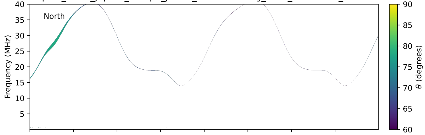
expres_earth_jupiter_europa_jrm33_lossc-wid1deg_3kev_20121115_v11.cdf
