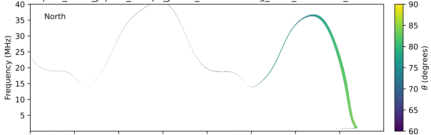
expres_earth_jupiter_europa_jrm33_lossc-wid1deg_3kev_20121112_v11.cdf
