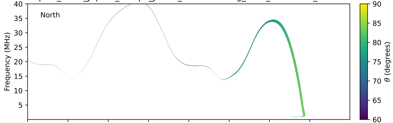
expres_earth_jupiter_europa_jrm33_lossc-wid1deg_3kev_20121105_v11.cdf
