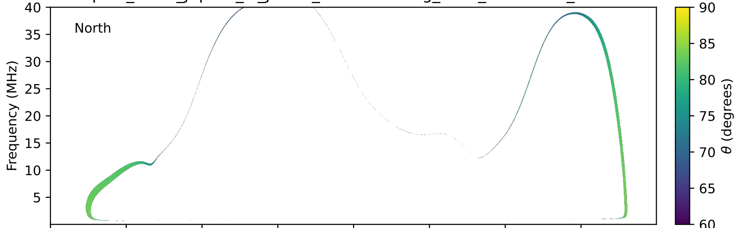
expres_earth_jupiter_io_jrm33_lossc-wid1deg_3kev_20121021_v11.cdf
