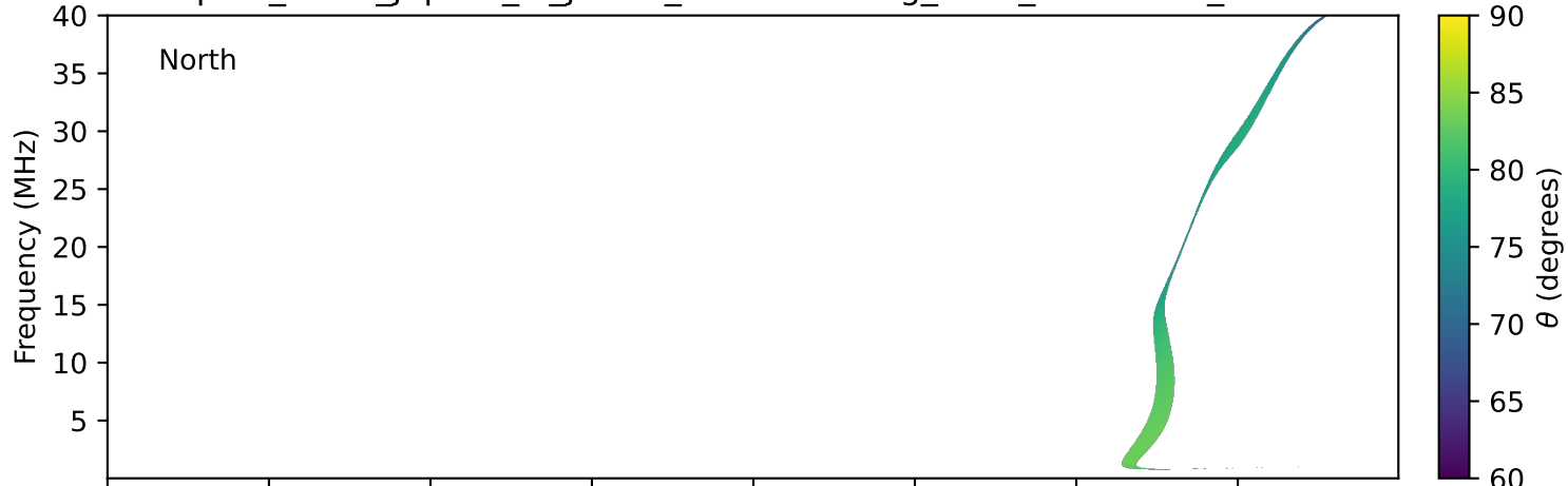
expres_earth_jupiter_io_jrm33_lossc-wid1deg_3kev_20121015_v11.cdf
