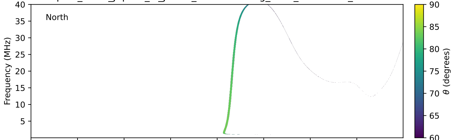
expres_earth_jupiter_io_jrm33_lossc-wid1deg_3kev_20121010_v11.cdf
