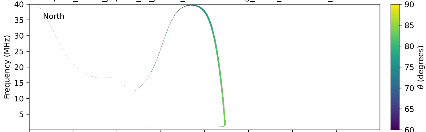
expres_earth_jupiter_io_jrm33_lossc-wid1deg_3kev_20121009_v11.cdf
