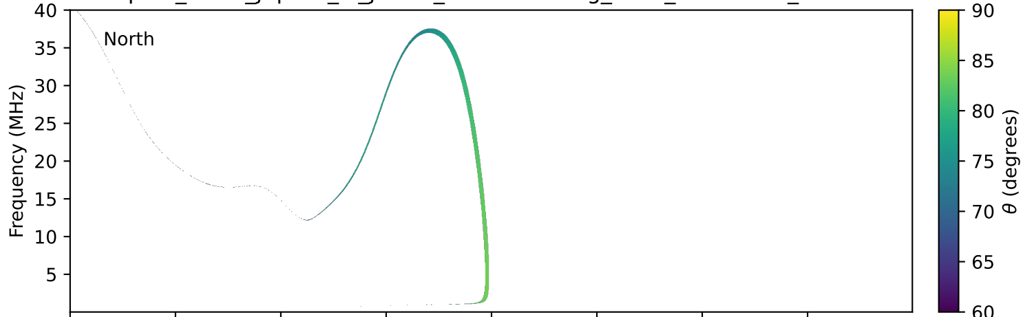
expres_earth_jupiter_io_jrm33_lossc-wid1deg_3kev_20121002_v11.cdf
