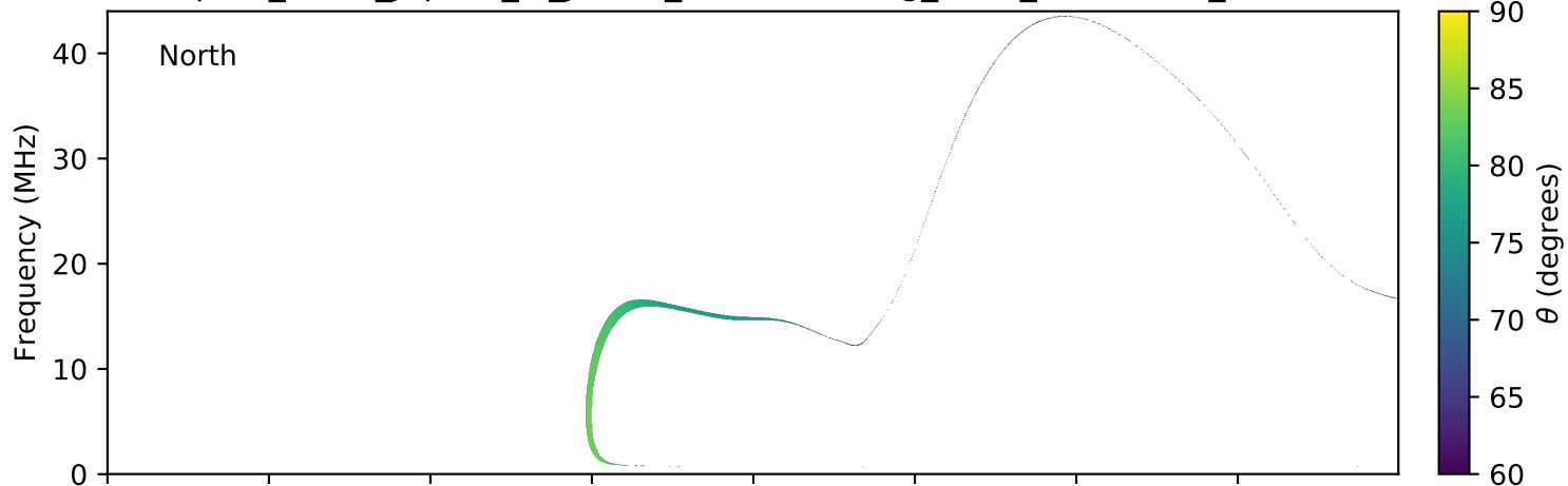
expres_earth_jupiter_io_jrm09_lossc-wid1deg_3kev_20121026_v01.cdf
