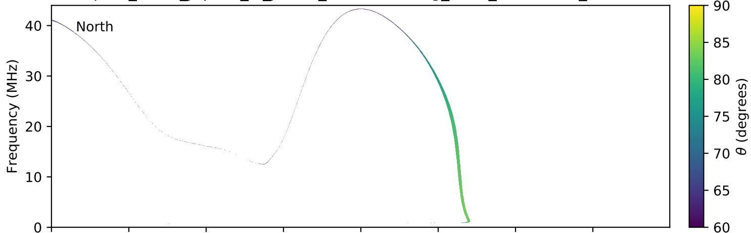
expres_earth_jupiter_io_jrm09_lossc-wid1deg_3kev_20121023_v01.cdf
