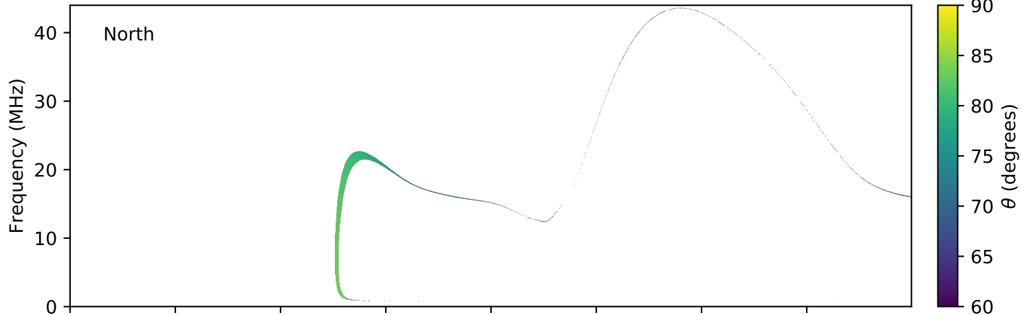
expres_earth_jupiter_io_jrm09_lossc-wid1deg_3kev_20121019_v01.cdf
