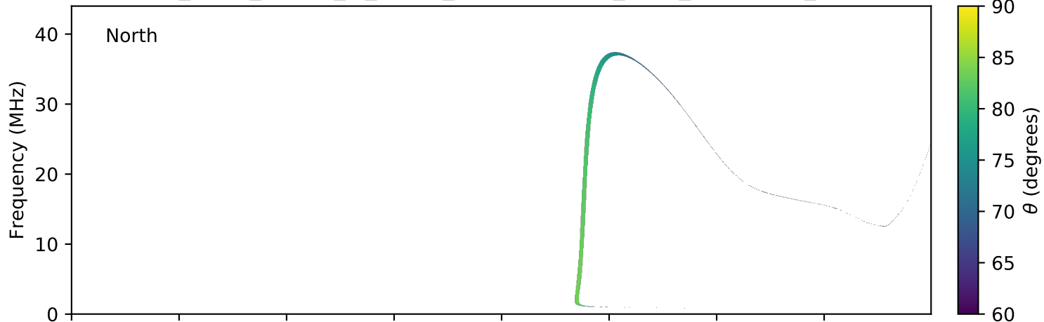
expres_earth_jupiter_io_jrm09_lossc-wid1deg_3kev_20121017_v01.cdf
