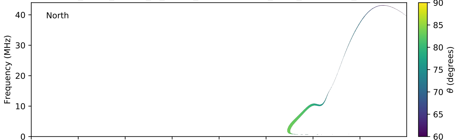
expres_earth_jupiter_io_jrm09_lossc-wid1deg_3kev_20121008_v01.cdf
