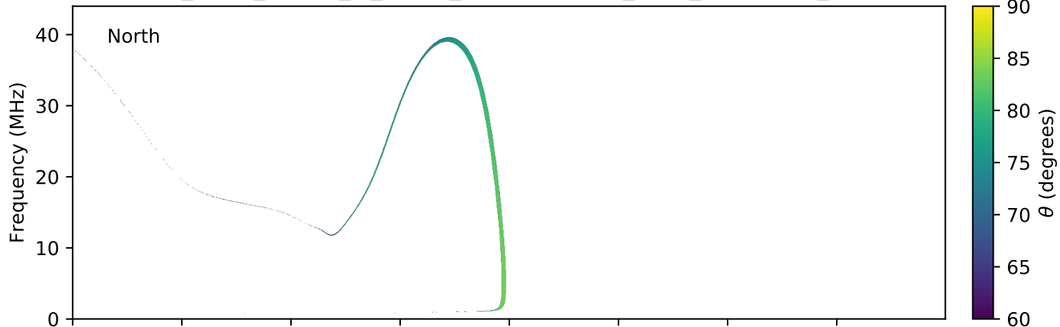
expres_earth_jupiter_io_jrm09_lossc-wid1deg_3kev_20121002_v01.cdf
