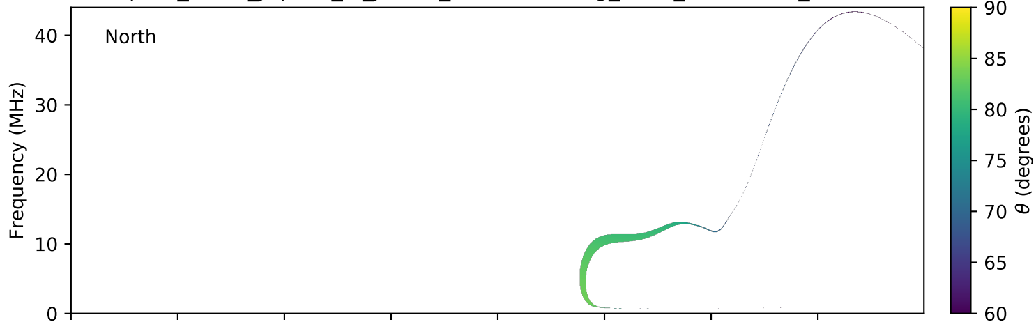
expres_earth_jupiter_io_jrm09_lossc-wid1deg_3kev_20121001_v01.cdf
