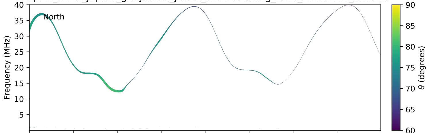
expres_earth_jupiter_ganymede_jrm33_lossc-wid1deg_3kev_20121030_v11.cdf
