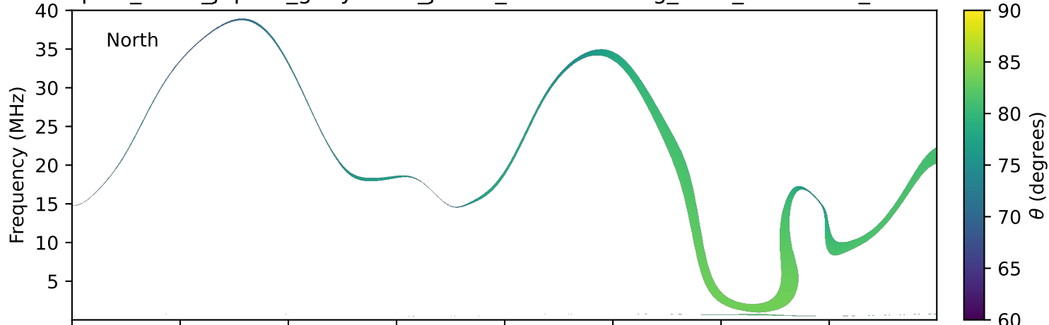
expres_earth_jupiter_ganymede_jrm33_lossc-wid1deg_3kev_20121025_v11.cdf
