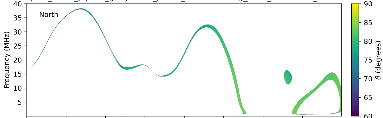
expres_earth_jupiter_ganymede_jrm33_lossc-wid1deg_3kev_20121018_v11.cdf
